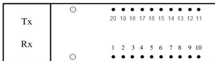
Figure 1 Pin out Drawing (Top view)
