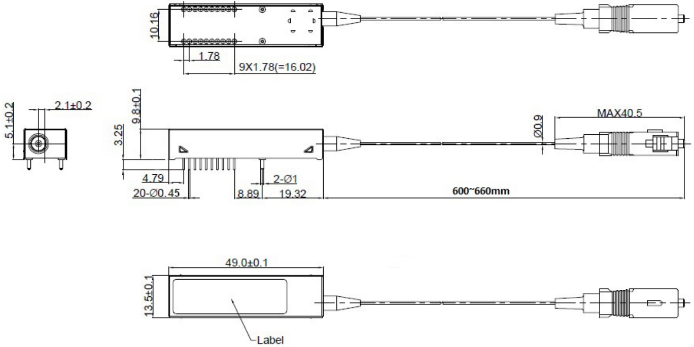
Figure 4 Package Outline
